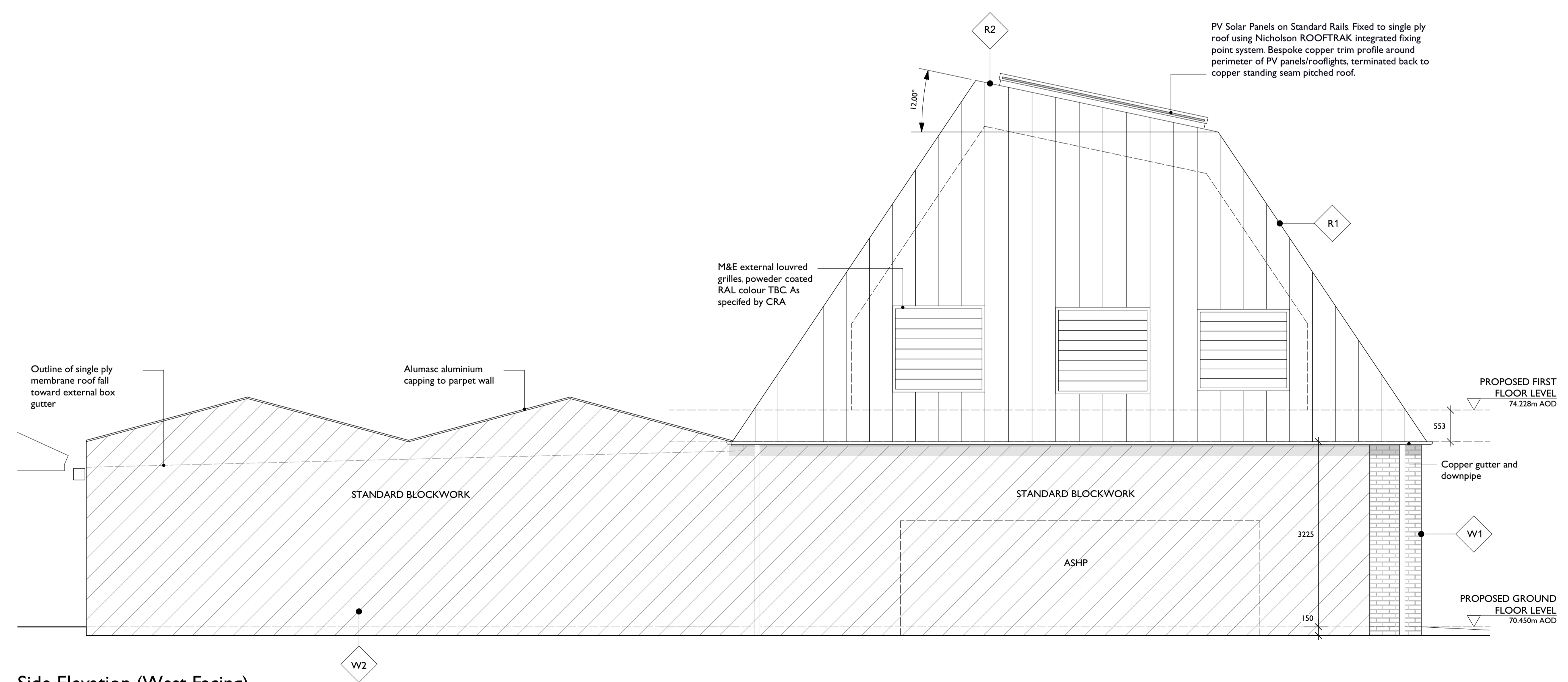
Side Elevation (West Facing)
