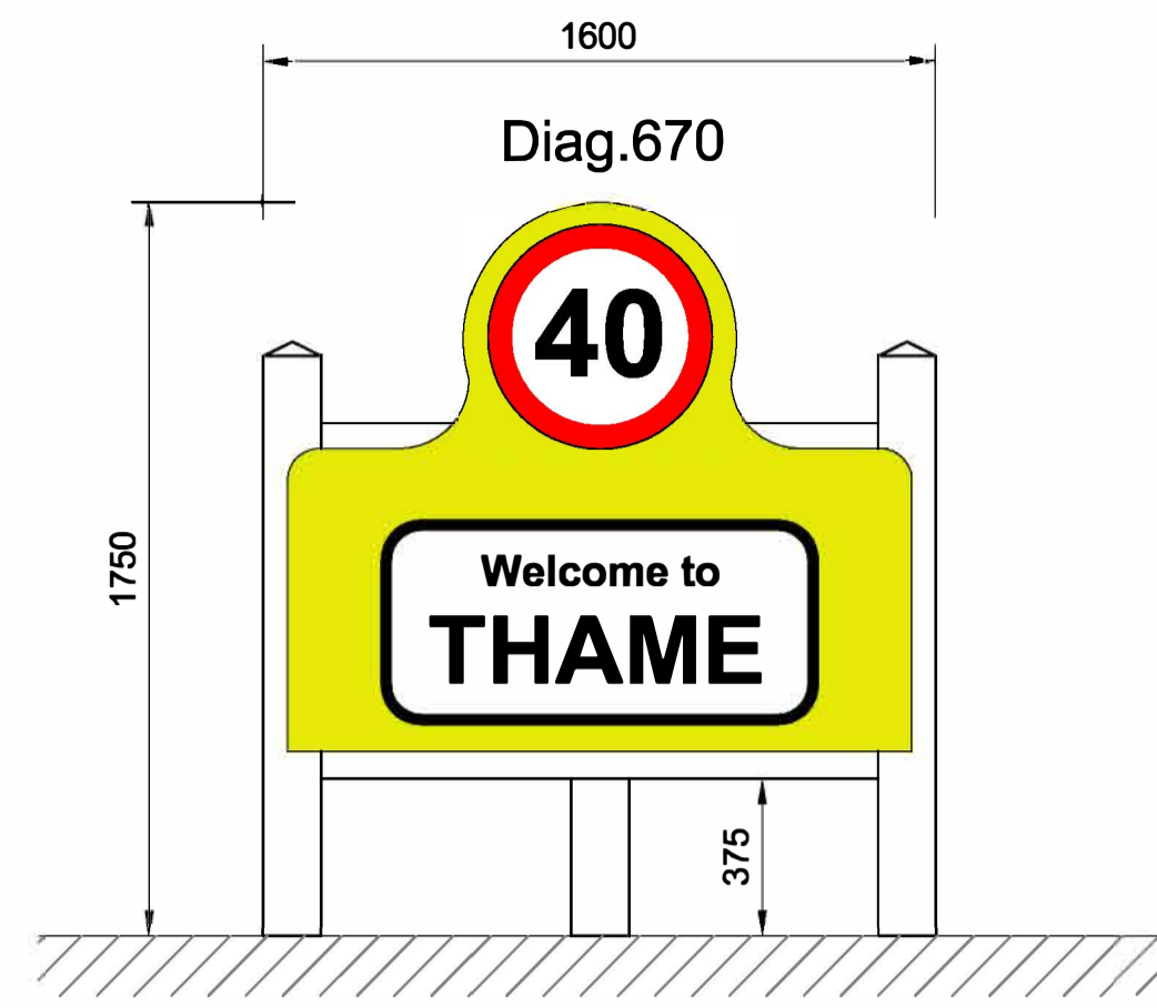
Village Gateway Sign 1:20
